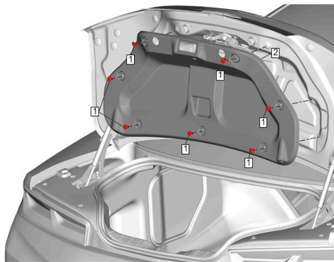
Figure 3: Rear Compartment Lid Inner Panel Trim Replacement
